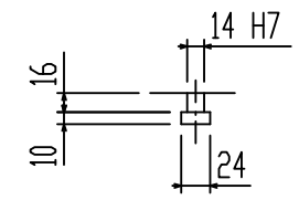
DETAIL OF T-SLOT
